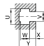
Partial view of T slot
